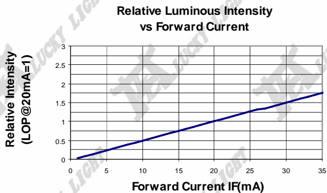
Relative Luminous Intensity vs Forward Current
