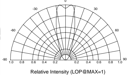
Beam Pattern
